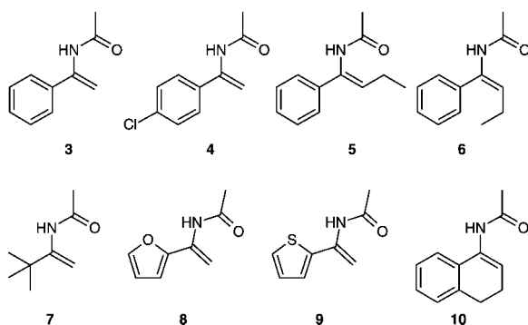
Figure 2. N -Acetyl- \alpha -arylenamide substrates.
