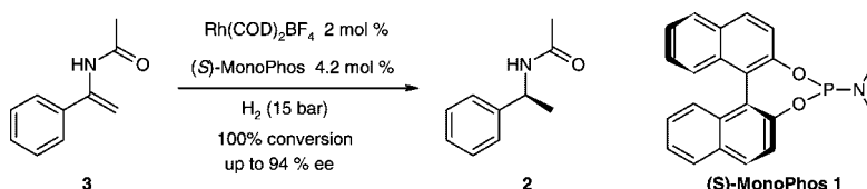
Scheme 1. Hydrogenation using monodentate phosphoramidite MonoPhos 1 .
