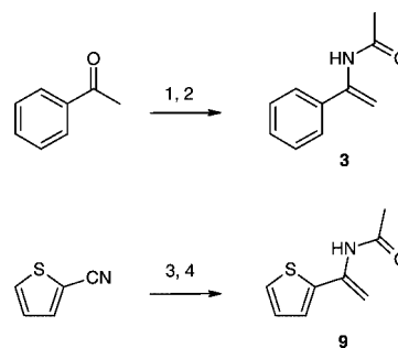
Scheme 2. Synthesis of substrates; [11,13,20,28] 1: \text{H}_2\text{NOH HCl} , EtOH, pyridine; 2: \text{Ac}_2\text{O} , AcOH, Fe, TMSCl, toluene; 3: MeMgBr, \text{Et}_2\text{O} ; 4: \text{Ac}_2\text{O} , \text{Et}_2\text{O} .
