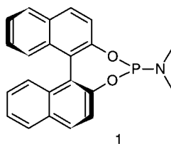
Figure 1. Monodentate phosphoramidite ligand MonoPhos 1 . [27,30]
